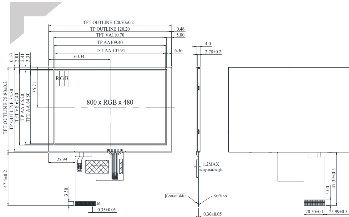
TFT INTERFACE
